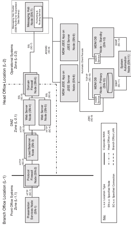
Figure 11.4 Multi-tier high availability for Critical Data Pattern for Transactional Hub deployment
