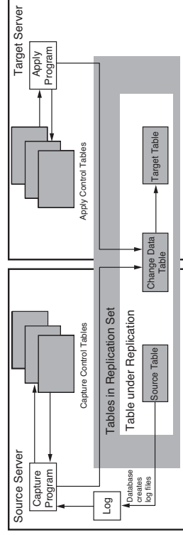
Figure 8.5 SQL replication
