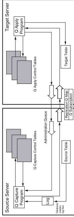
Figure 8.6 Queue replication
