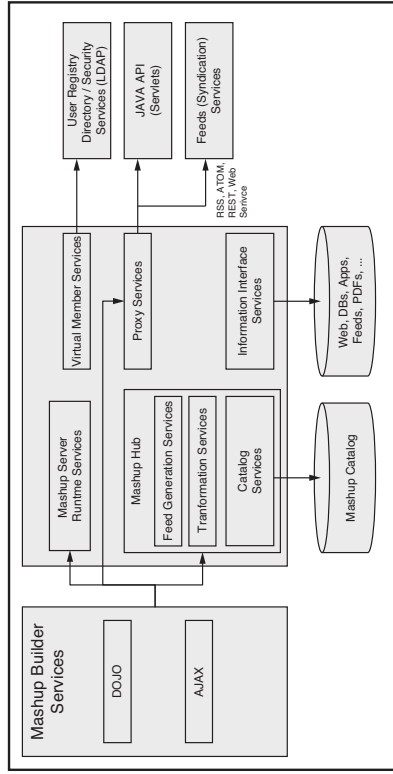
Figure 12.3 Architecture overview
