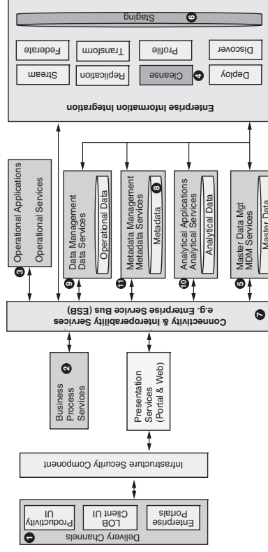
Figure 8.3 Cleansing scenario
