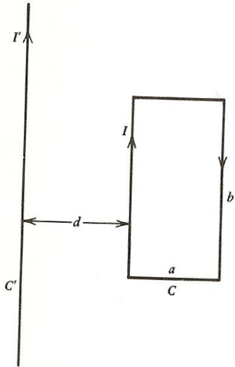
Figure 13-5. The circuits of Exercise 13-4.
