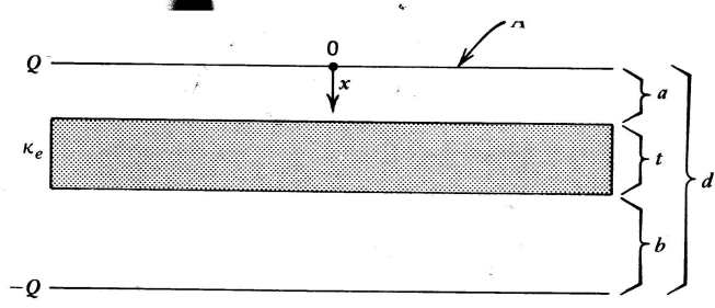
Figure 10-19. Capacitor in Exercise 10-23.
