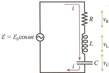
FIGURE 36.17 A series RLC circuit.
