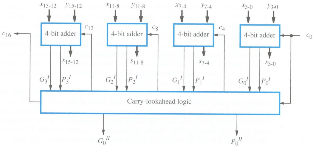
Figure 6.5 16-bit carry-lookahead adder built from 4-bit adders
